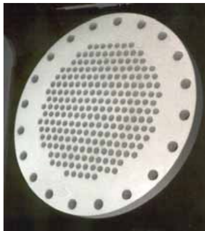
PACKING SUPPORT PLATE 22" diameter, RTFE
